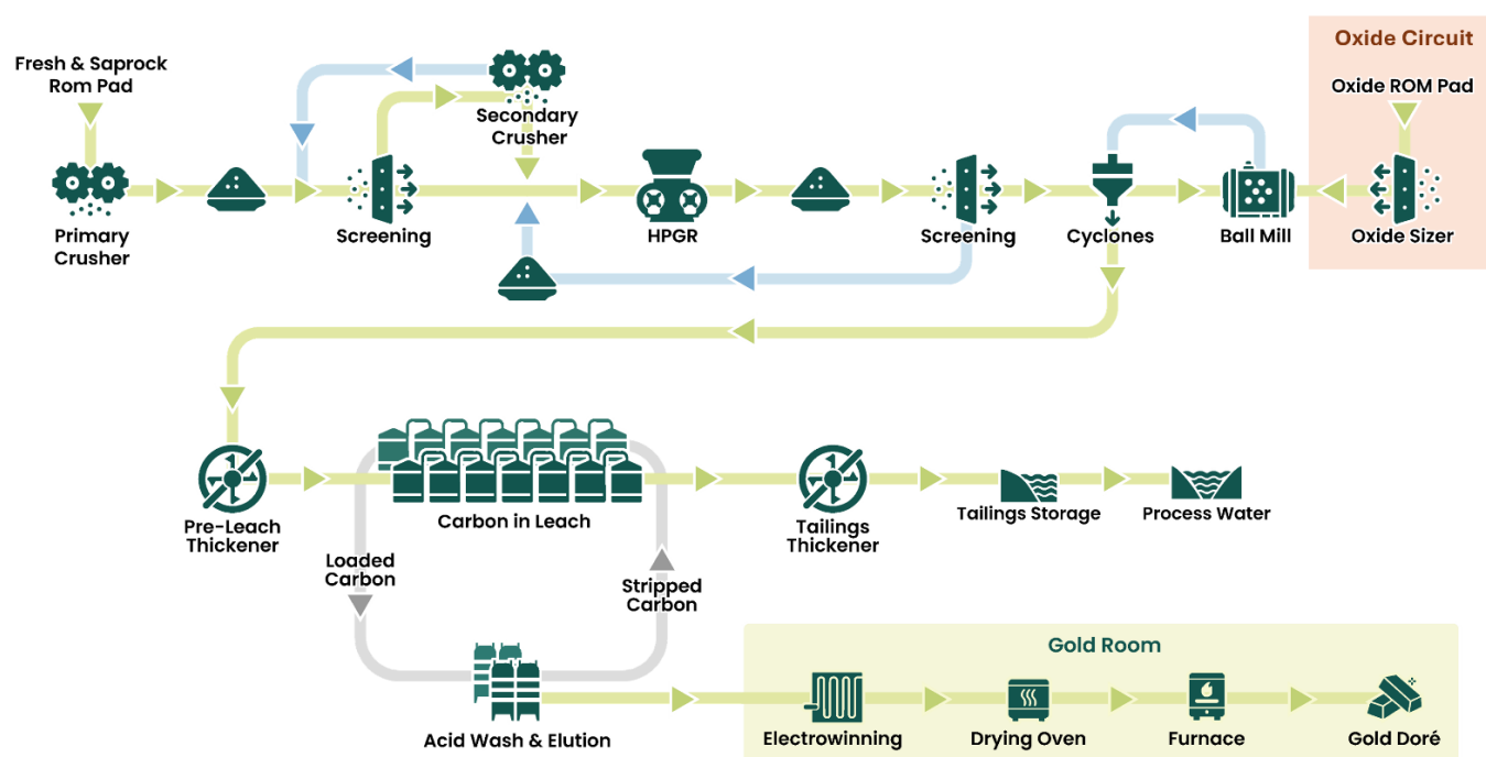
Figure 3: Koné processing plant flowsheet with oxide circuit
